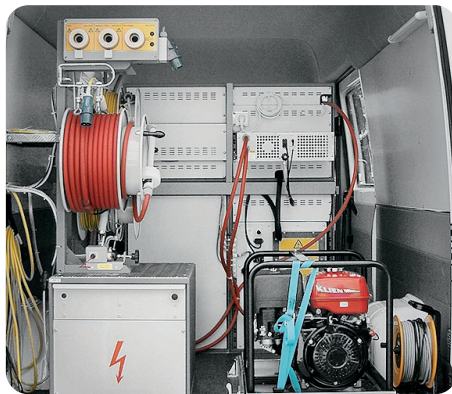
The transcable system ↑
